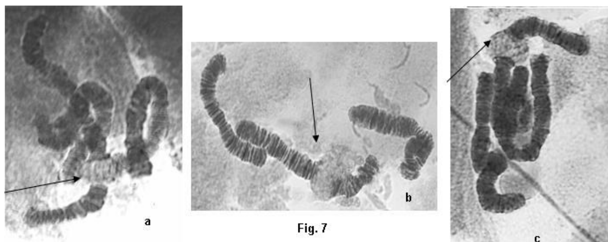
Figure 7. Different Balbiani rings on chromosome I, revealing gene activation timing (a,b and c) in Chironomus plumosus (100x)
